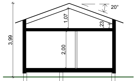
S1 Sovrum-WC-Loft 1:100
